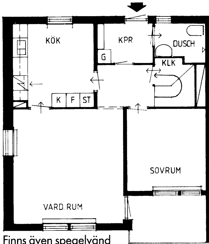
underplan
